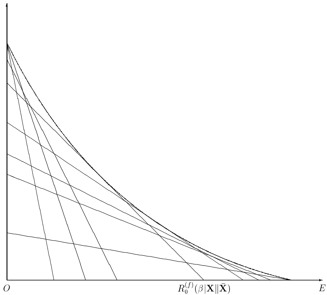
Figure 5.5: Convex lower bound for testing between arbitrary Markov sources. Each line of slope \beta intersects the E -axis at R_0^{(f)}(\beta|\mathbf{X}||\bar{\mathbf{X}}) . Proceeding from left to right, the values of \beta are: -5, -3, -2, -1, -2/3, -1/2, -2/5, -1/6 .
